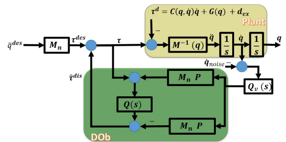
Fig. 3: Block diagram of DOB internal loop
