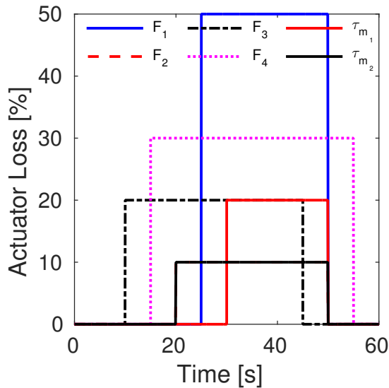
Fig. 5: Actuators Loss
